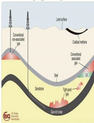
Schematic geology of natural gas resources
